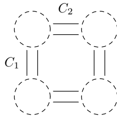
Figure 4: Two interlaced 4-cuts.
