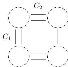
Figure 3: A 3-cut C_1 interlaced with a 4-cut C_2 .
