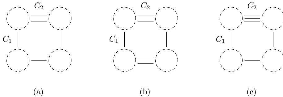
Figure 2: A 2-cut C_1 (vertical edges) interlaced with a cut C_2 of size 3 or 4 (horizontal edges).
