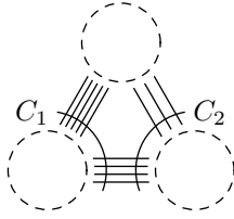
Figure 5: Non-interlaced cuts C_1 and C_2 with common edges.
