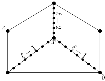
Figure 10: A graph that is not \ell -facial colourable with 3\ell - 1 colours
