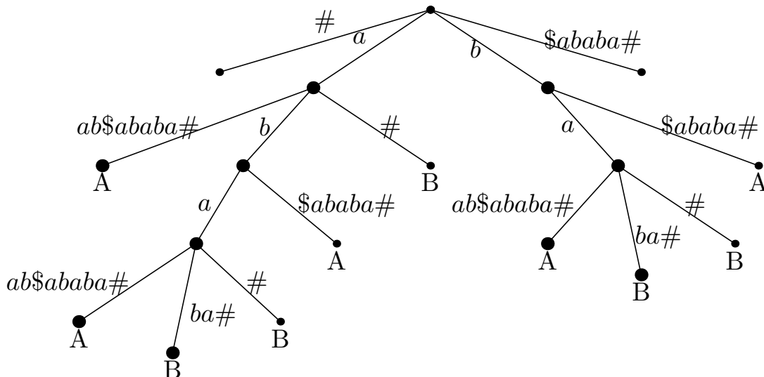
Figure 2: Suffix tree \tau of the string C = abaab\$ababa\# . The larger dots denote the proper nodes.
