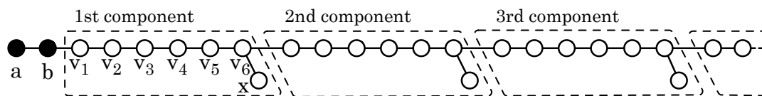
Figure 9: The graph G_l used to prove the lower bound.
