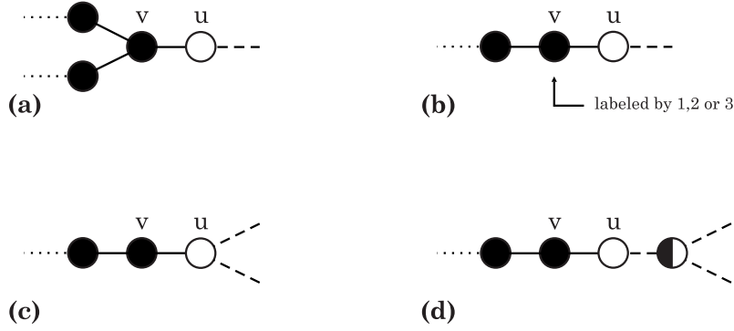
Figure 2: Forced extensions.
