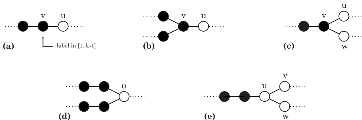
Figure 10: Simple branchings.
