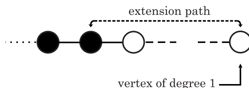
Figure 3: Easy extension. An extension path with one unlabeled endpoint of degree 1.
