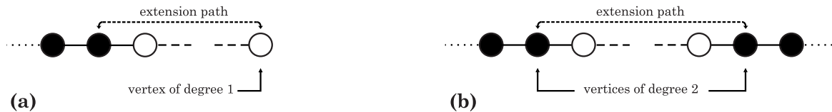
Figure 11: Cheap extensions. (a) An extension path with one unlabeled endpoint of degree 1. (b) An extension path with both endpoints labeled and of degree 2.
