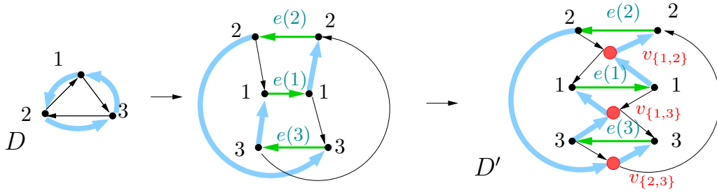
FIGURE 2. An example of the construction of D' from D
