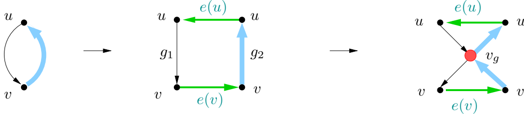
FIGURE 1. Construction of e(v) and v_g
