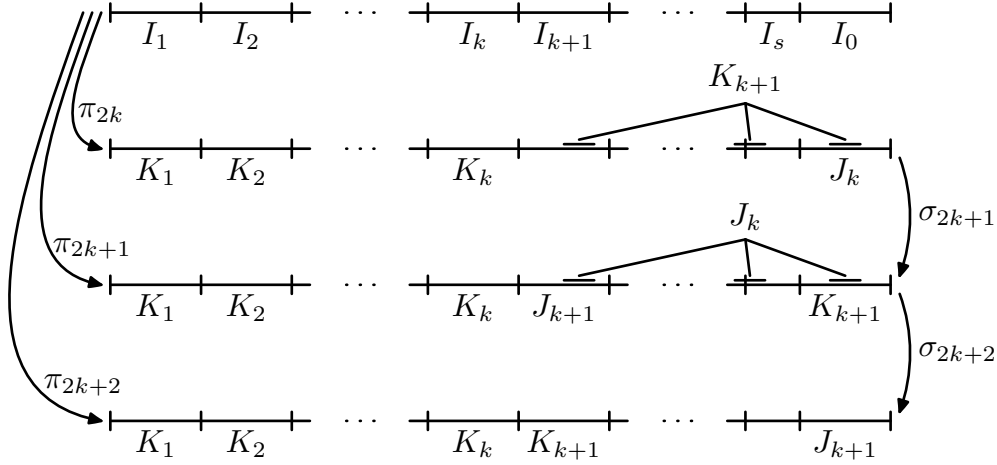
Figure 1: An illustration of the actions of the isometries \pi_{2k+1} and \pi_{2k} . The colors in K_{k+1} are not used on level 2k + 1 , and the colors in J_{k+1} are not used on level 2k + 2 . Moreover, \pi_{2k} and \pi agree on I_1 \cup \dots \cup I_k .
