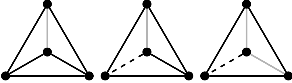
FIGURE 2. Representative elements of \mathcal{H}(2, 1, 0) , \mathcal{H}(1, 1, 1) and \mathcal{H}(0, 2, 1) .
