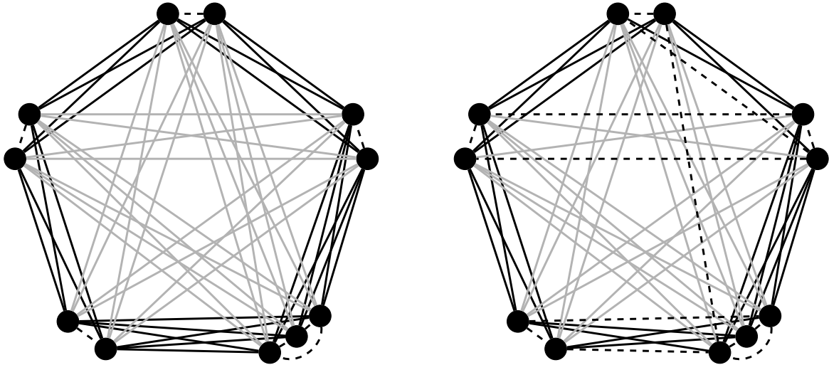
FIGURE 1. G_{ex}(11) and another element of \mathcal{G}_{11}
