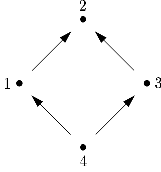
Figure 1: Partially ordered set P
