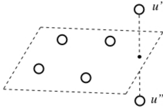
Figure 5. Blowing a vertex of the pentagon.
