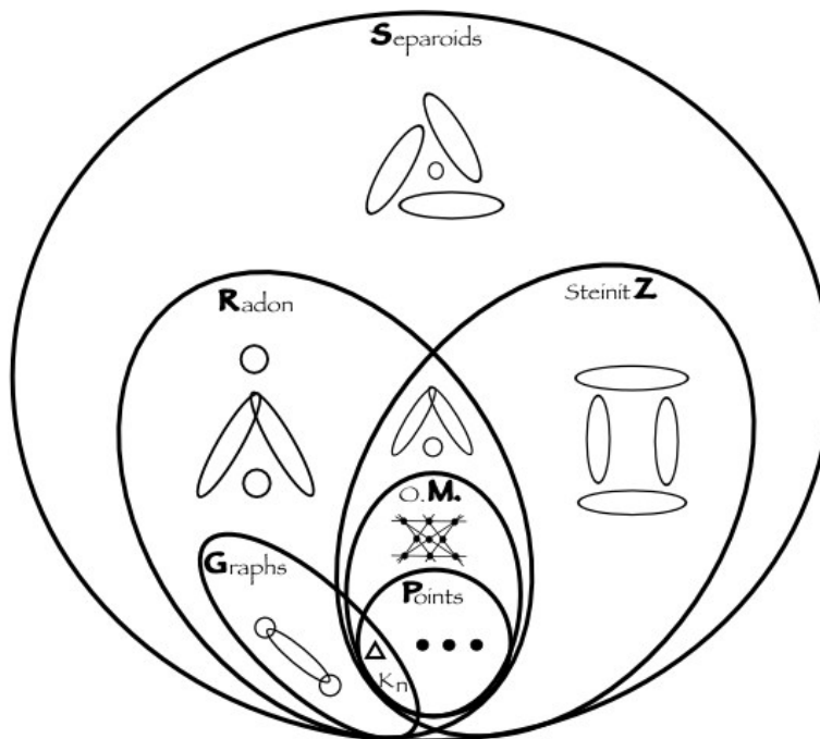
Figure 2. Some classes of separoids.
