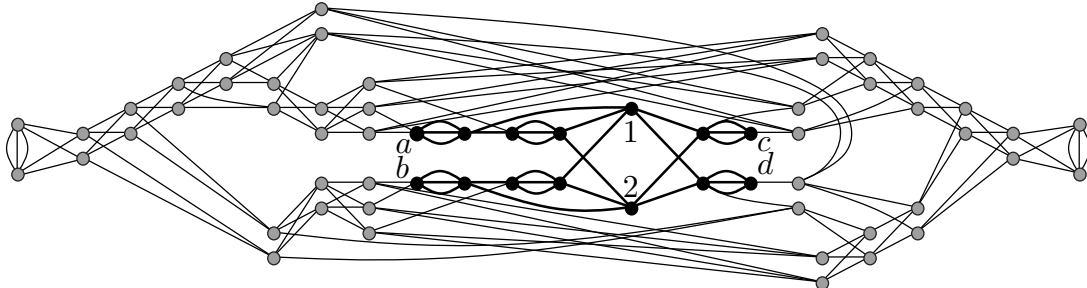
Fig. 4. Constructed 5-regular multigraph for formula (a \vee a \vee b \vee c \vee d) \wedge (a \vee b \vee b \vee c \vee d) . Clause vertices are marked 1 and 2. Clause vertices and variable paths are drawn in black colour, vertices p_i^x and vertices added by the procedure are in gray colour.
