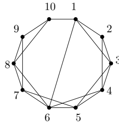
Figure 2: Pavol's rigid graph
