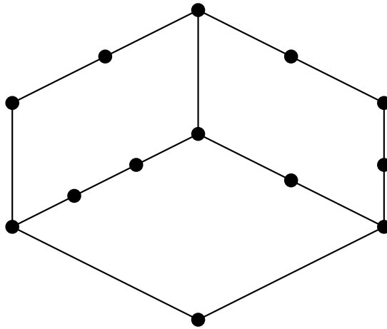
Figure 1: Hedrlín Pultr graph [63]
