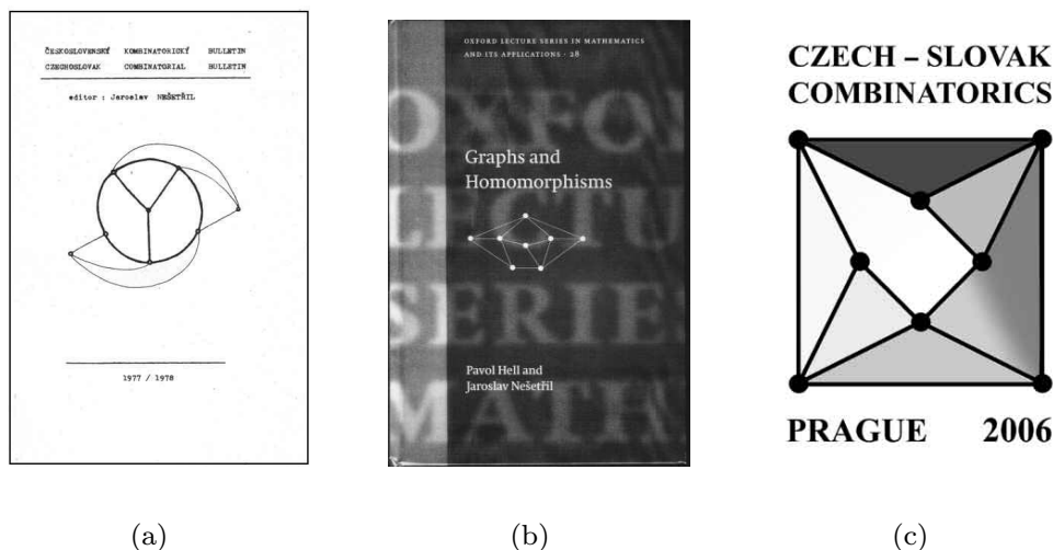
Figure 5: Reproducing Our Graph
