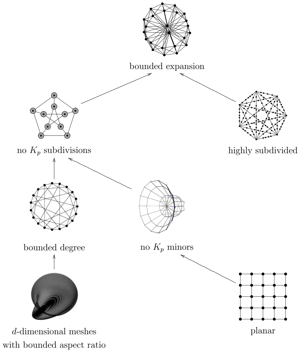
FIGURE 3.1. Classes with Bounded Expansion
