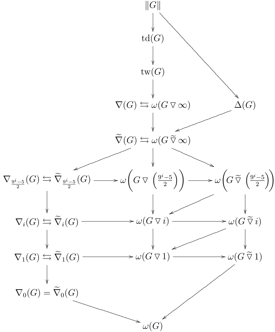
FIGURE 2.3. Dominance of Invariants (up to polynomial transformation)
