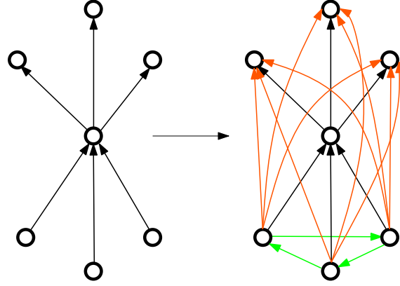
FIGURE 4.4. The Transitive Fraternal Augmentation of a Graph
