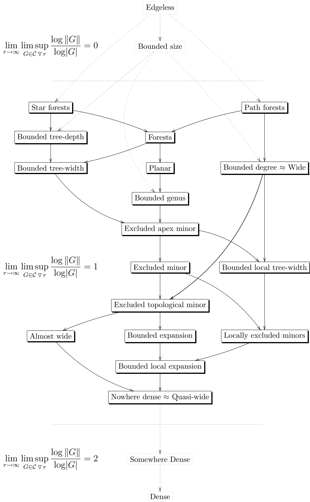
FIGURE 3.2. The Nowhere Dense World: inclusion map of some important properties of hereditary classes of graphs.
