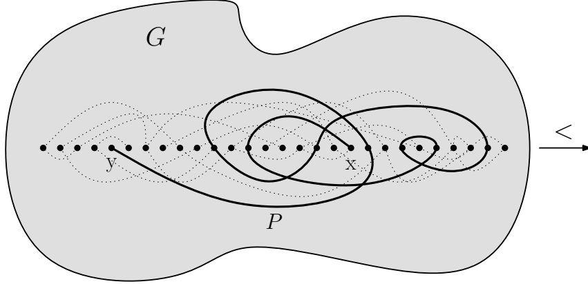
FIGURE 4.2. The vertex y is weakly 8-accessible from x
