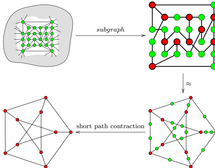
FIGURE 3. A Petersen topological minor of depth 1 in a graph
