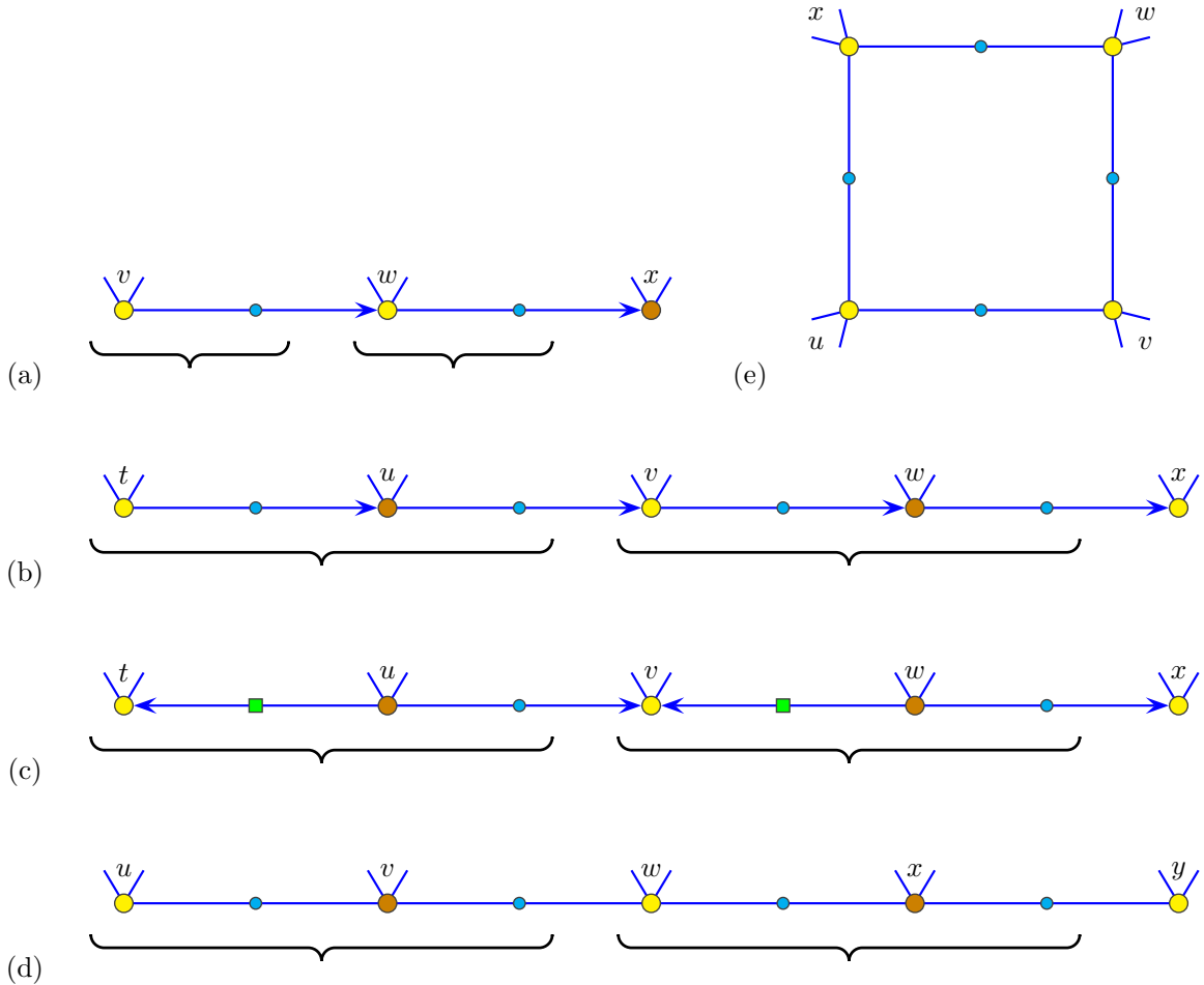
FIGURE 6. Illustration for Lemma 9.6.
