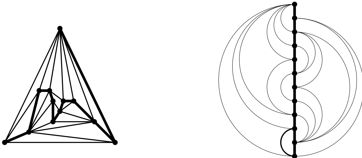
FIGURE 4. Every 4-connected planar graph has stack number at most 2 (since it is Hamiltonian)
