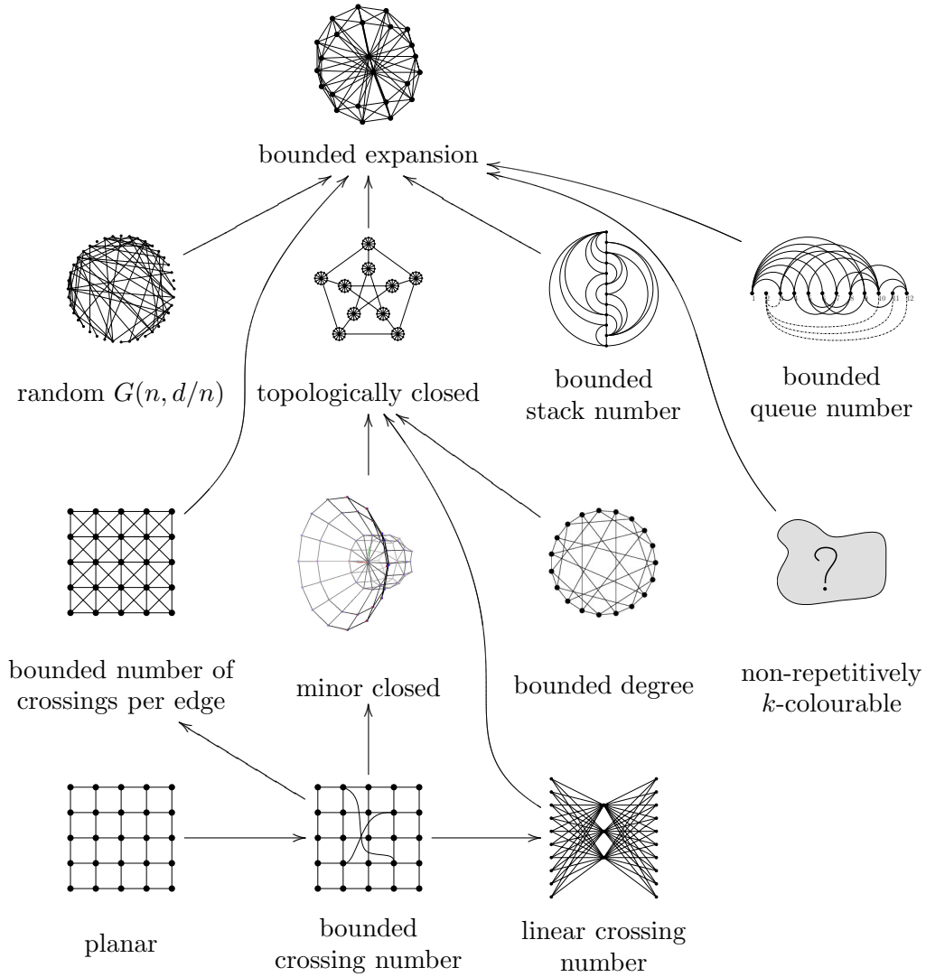
FIGURE 1. Classes with Bounded Expansion. The results about classes with bounded crossings, bounded queue-number, bounded stack-number, and bounded non-repetitive chromatic number are proved in this paper.
