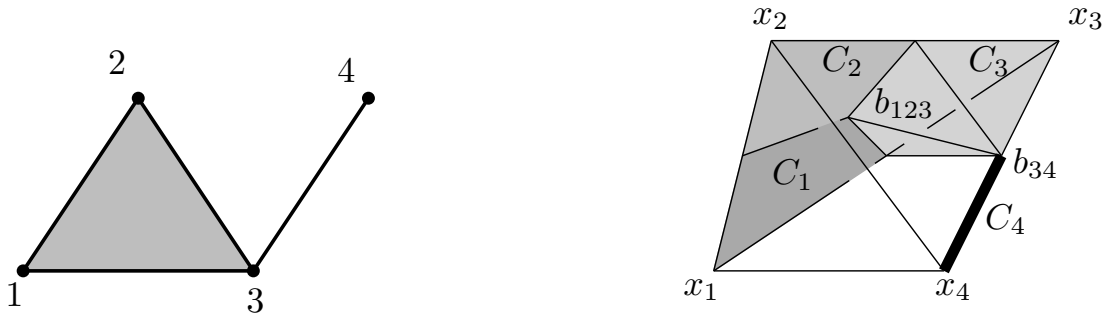
Figure 4: Representing a complex.
