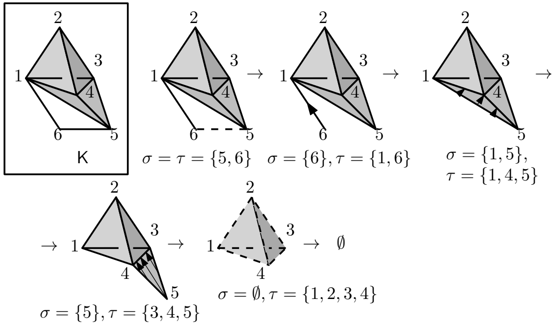
Figure 2: A 2-collapsing of a simplicial complex.
