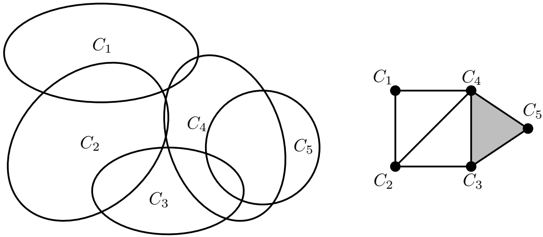
Figure 1: A 2-representable complex and its nerve.
