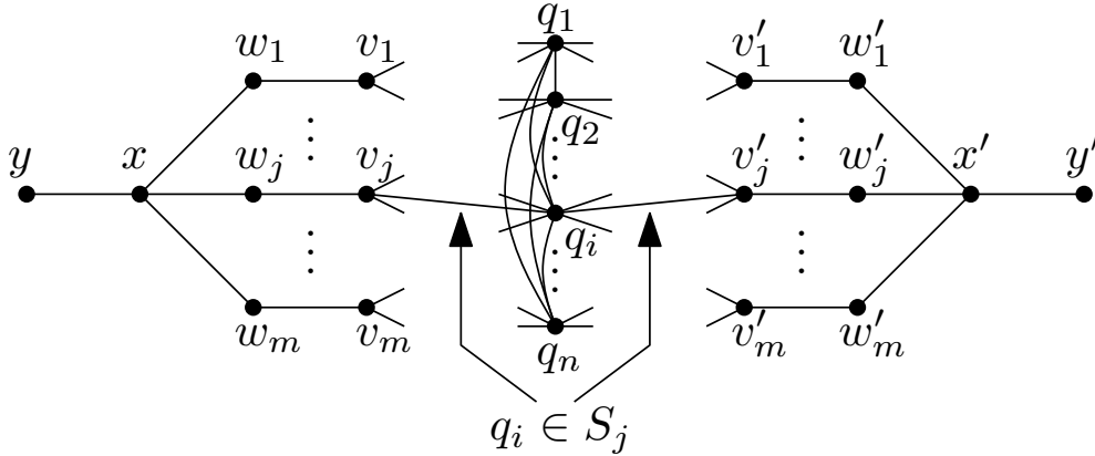
Fig. 1. The constructed graph G .
