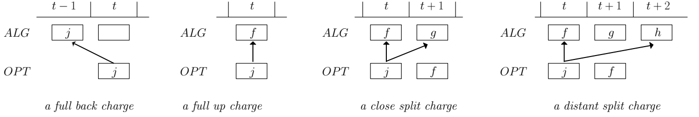
Figure 3: Non-chaining charges. Note that for split charges f is scheduled in step t + 1 in OPT which follows from the fact that we do not charge j using a full up charge.
