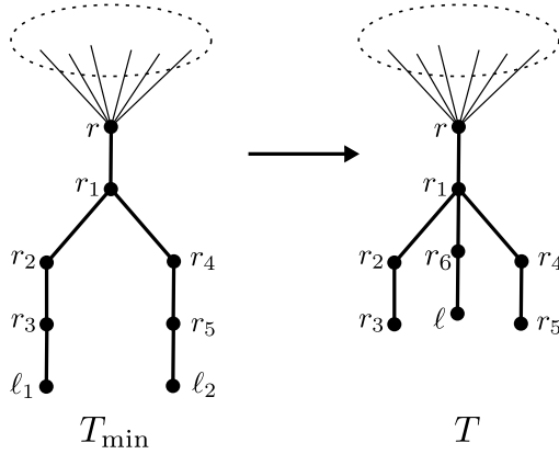
Figure 6. An illustration of construction in Proposition 5.
