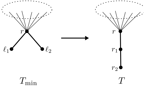
Figure 3. An illustration of construction in Proposition 2.
