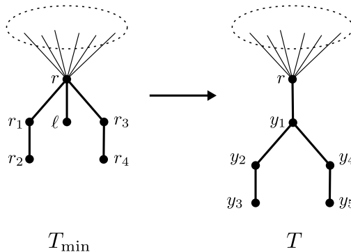
Figure 4. An illustration of construction in Proposition 3.
