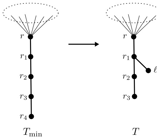
Figure 5. An illustration of construction in Proposition 4.
